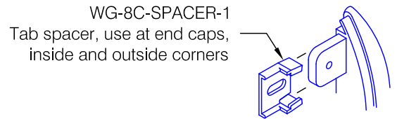
Spacer Detail
