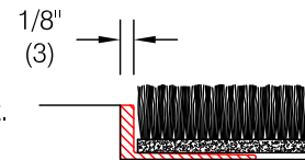
Recessed frame SSF-125 (see ED.3.0)
