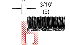
Recessed frame MRF-1002 (see ED.1.0) or MRF-1005 (see ED.2.0)
