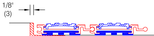
Recessed frame SSF-125 (see ED.3.0)
