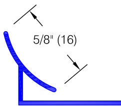
WCT-100 Inside corner 90° corner
