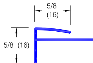
WCT-101 Outside corner
