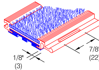
Optional perforated hinge (solid hinge standard)
