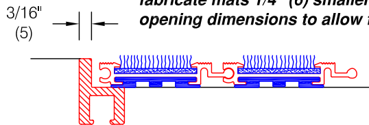
Recessed frame MRF-1002 (see ED.1.0) or MRF-1005 (see ED.2.0)
