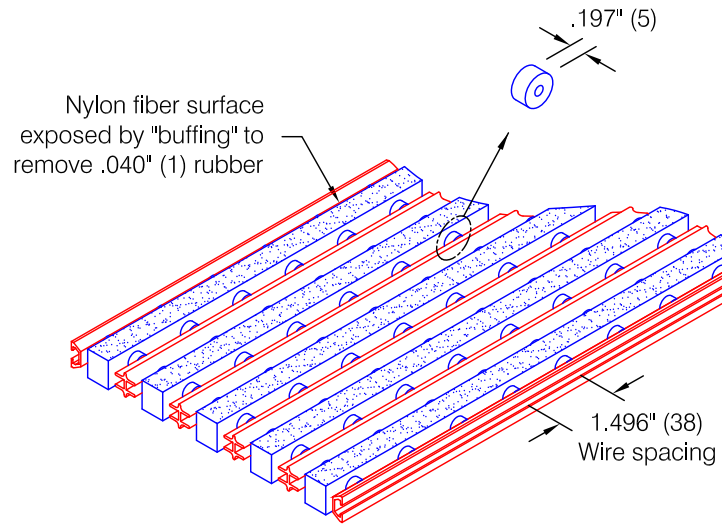
"OS" : Open Construction, Single Insert
