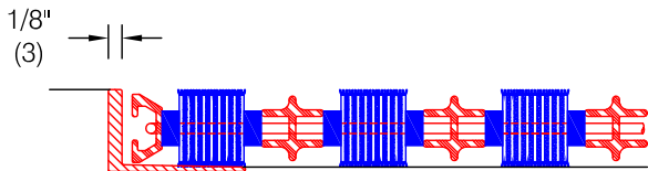
Optional recessed frame SSF-250, see ED.7.2
