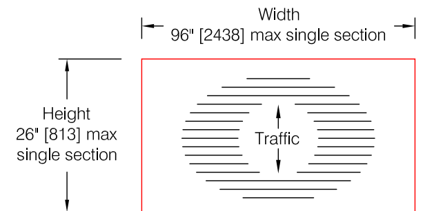
"OS" : Open Construction, Single Insert
