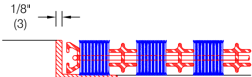
Optional recessed frame SSF-250, see ED.7.2
