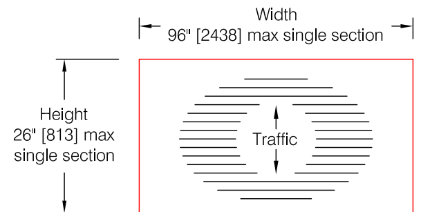
"CD" : Closed Construction, Double Insert
