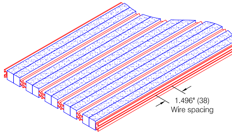
"CD" : Closed Construction, Double Insert
