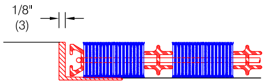
Optional recessed frame SSF-250, see ED.7.2
