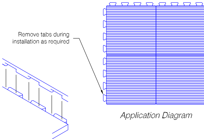
Interlocking Tab Detail
