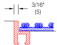
Recessed frame MRF-1002 (see ED.1.0) or MRF-1005 (see ED.2.0)
