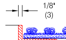
Recessed frame SSF-125 (see ED.3.0)
